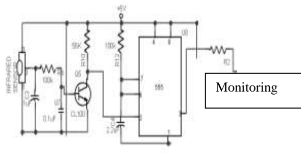
Figure 2. Pulse rate Detection Circuit
